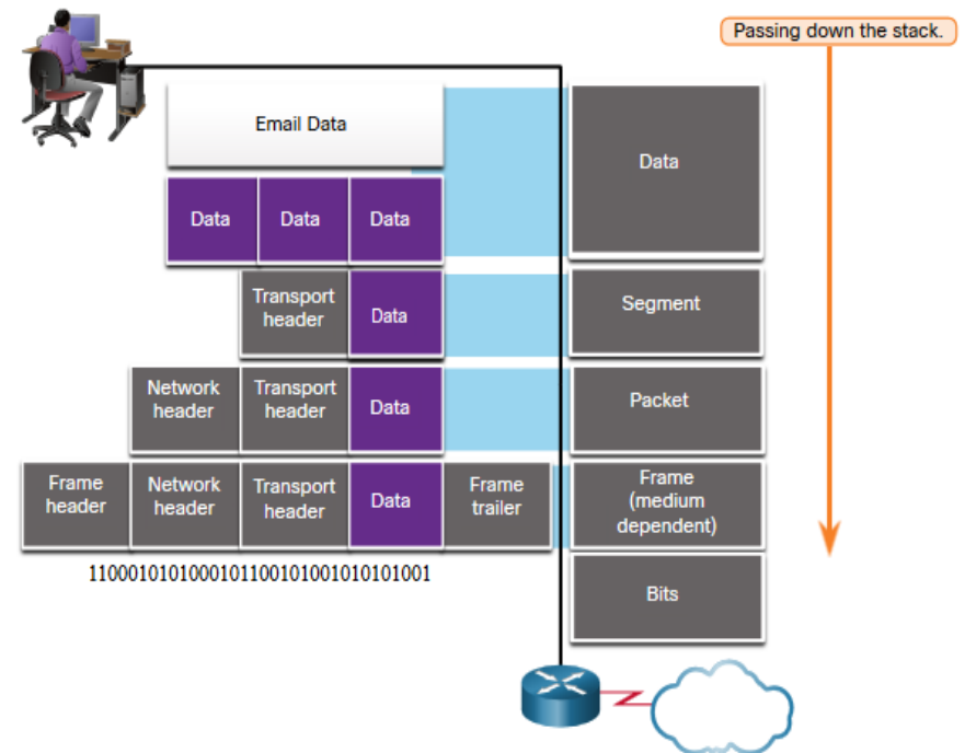
Protocol Data Unit (PDU)
